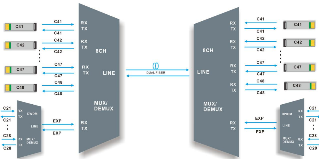
8CH DWDM MUX DEMUX Dual fiber transmission
