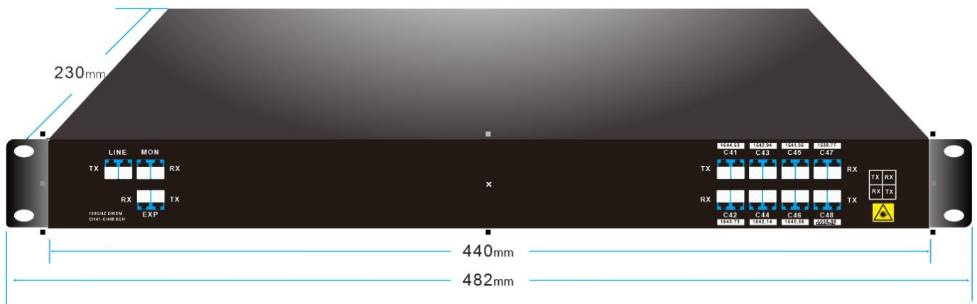
19" Inch 1U Rack
