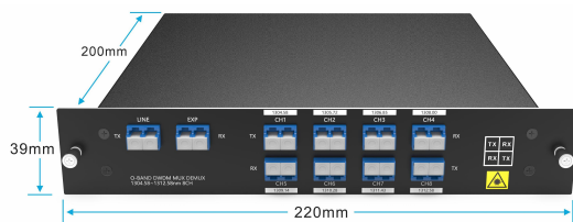
LGX BOX Plug in 2-Slot 1U Rack
