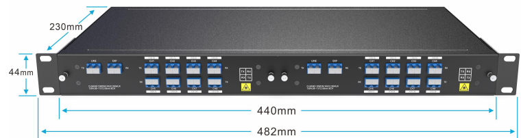
2-Slot 1U Rack for LGX BOX
